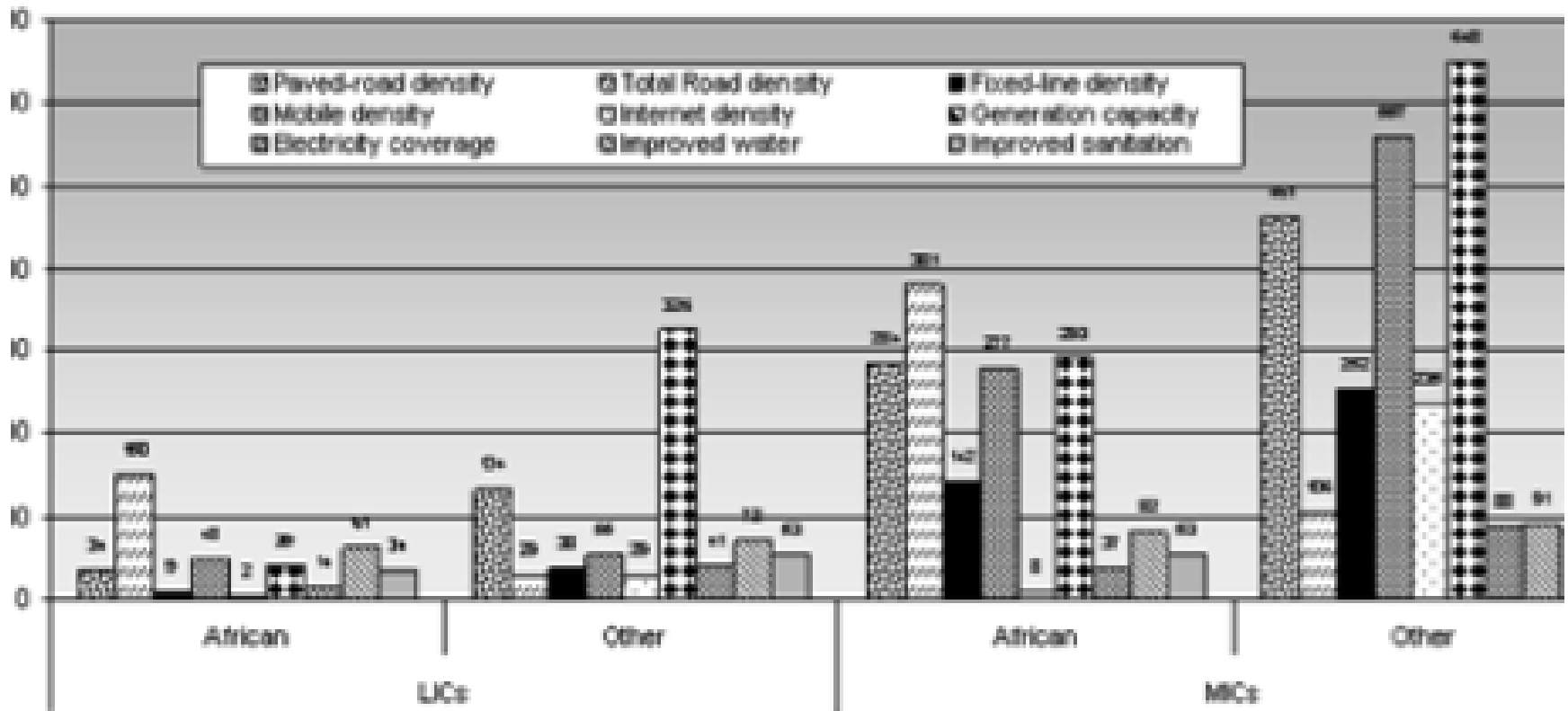
Figure 4: International Comparisons of Infrastructure Supply Conditions
